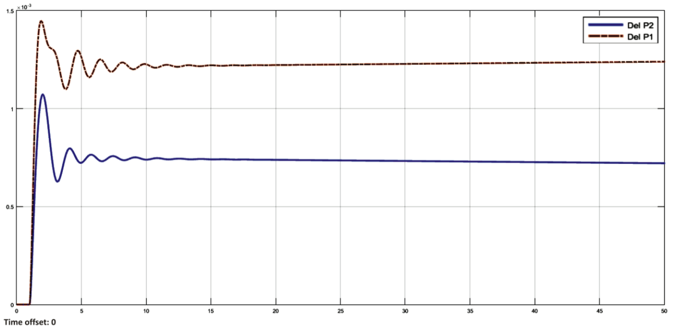
Figure 9: Change in power using a PI controller
