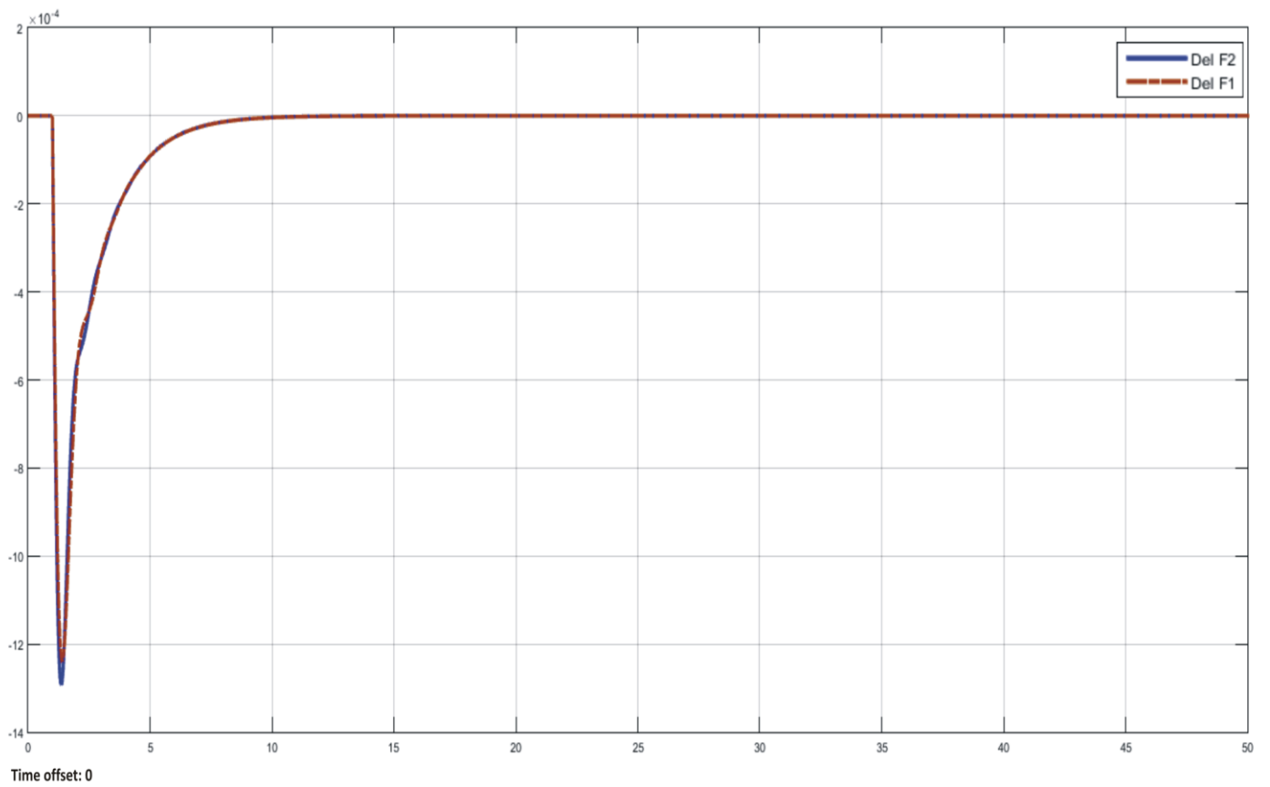
Figure 7: Change in frequency using a fuzzy logic controller
