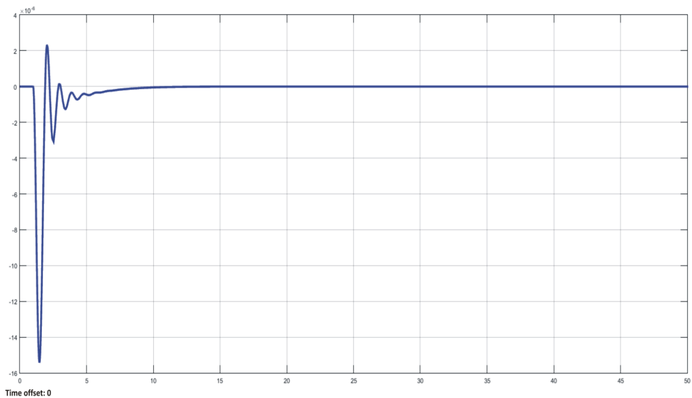
Figure 13: Power deviation in tie line using a fuzzy logic controller
