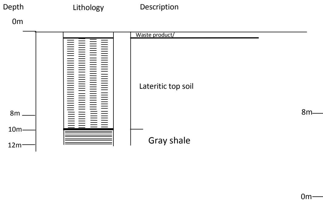
Fig. 2. Lithostratigraphic section of oke-diya dumpsite
