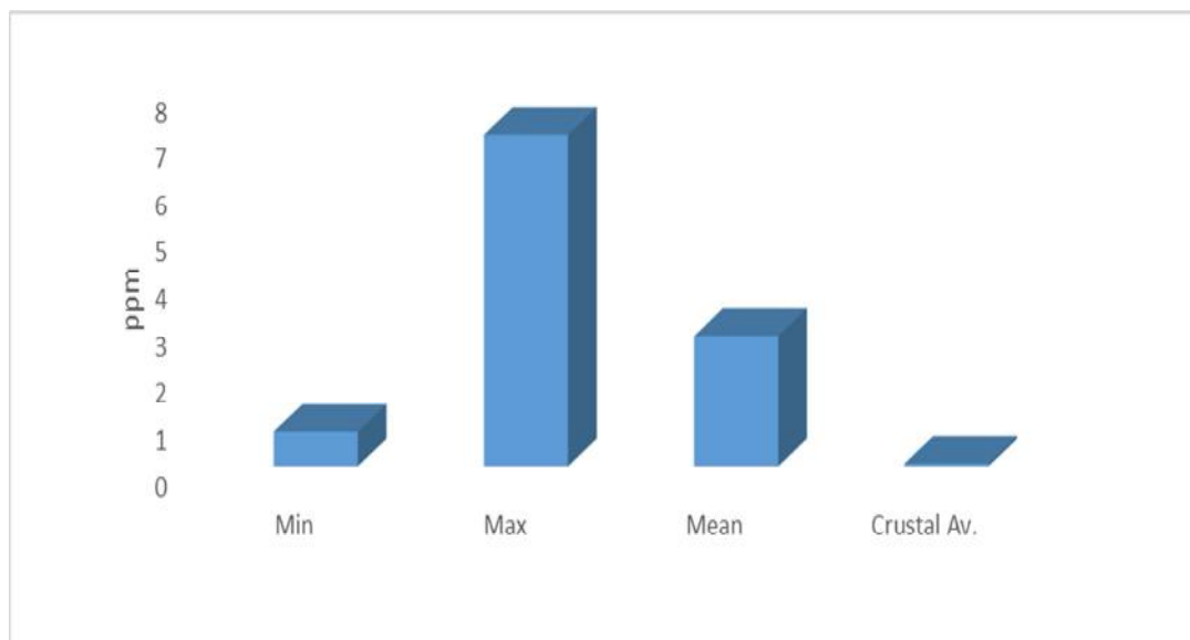
Fig. 3b. Plot of summary of Fe with crustal average
