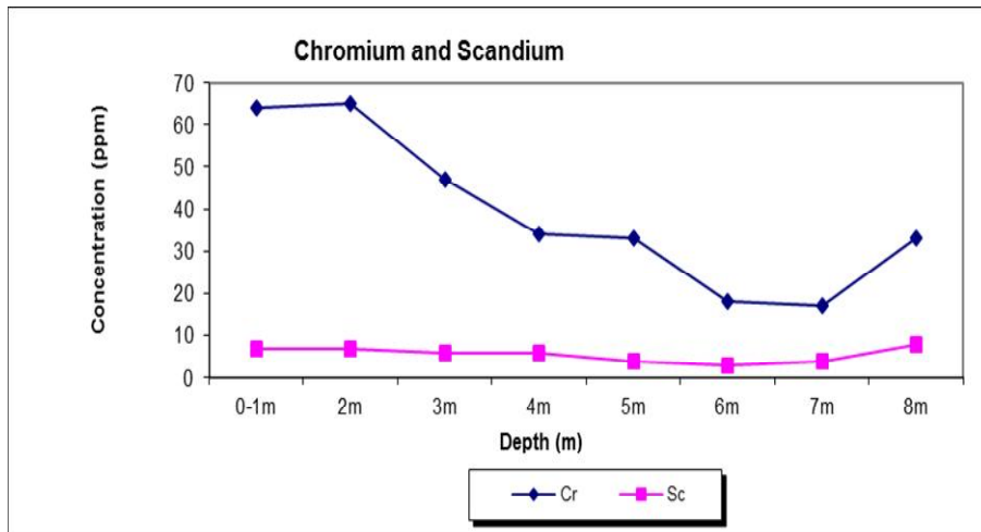
Fig. 5a. Concentration of trace elements in soil sample at different depth interval
