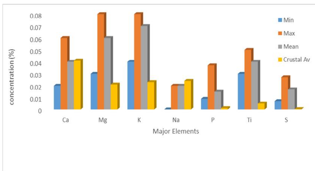
Fig. 3a. Plot of summary of major elements with ASC
