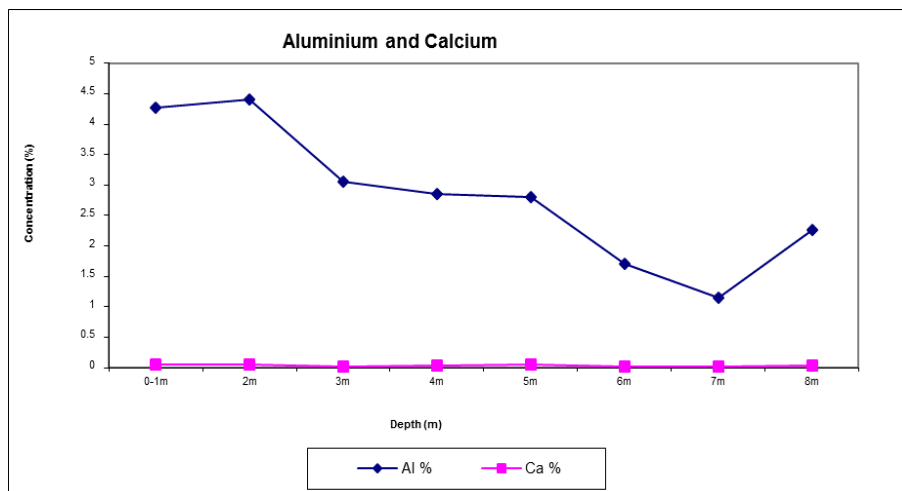
Fig. 5c. Concentration of trace elements in soil sample at different depth interval
