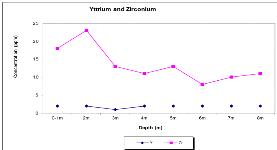
Fig. 5b. Concentration of trace elements in soil sample at different depth interval
