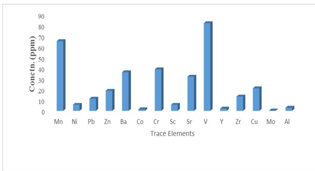
Fig. 4. Plot of mean values of trace elements
