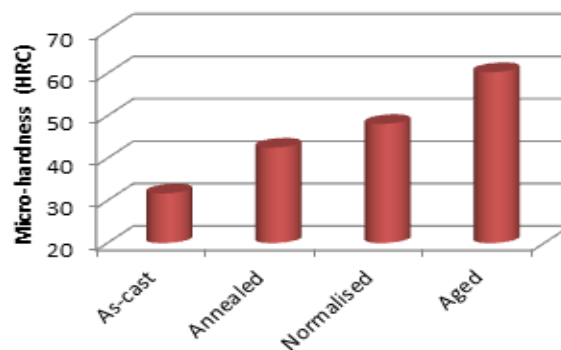
Fig. 5 Variations of micro-hardness developed by test specimens
