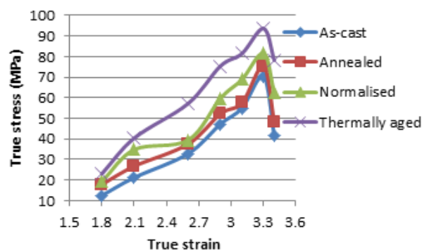
Fig. 2 True stress-strain graph of test specimens
