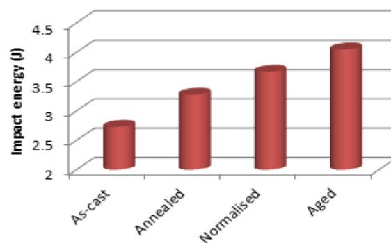
Fig. 4 Impact energy variations of test specimens
