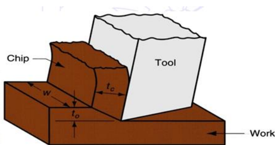
(a) as a three-dimensional process
