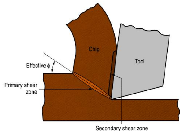
(b) showing shear zone rather than shear plane
