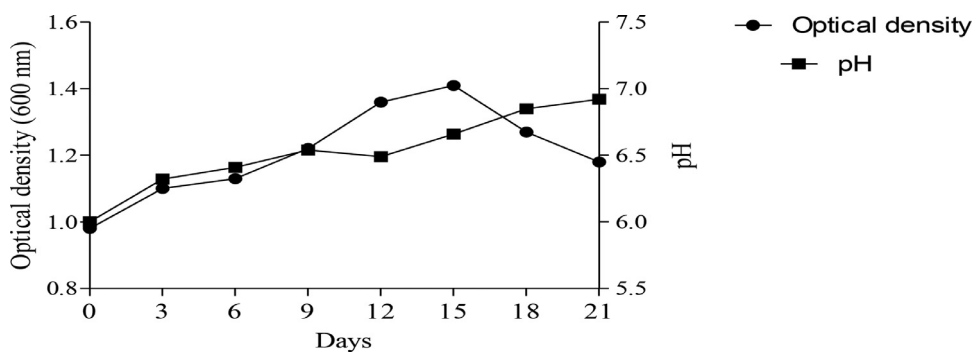
Fig 1. Growth profiles of pure cultures of Streptomyces coelicolor strain COB KF977550 in sugarcane bagasse as the carbon source.
