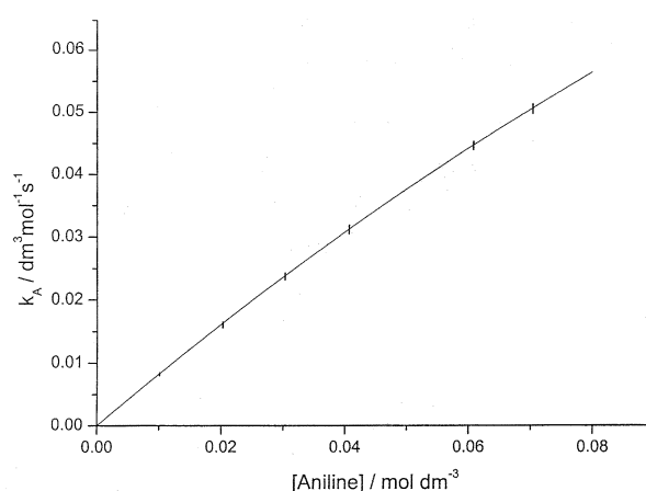
Fig. 1 Plot of k_A versus [aniline] in acetonitrile at 25 °C for the reaction of 4-bromophenyl 2,4,6-trinitrophenyl ether. Experimental values are denoted by |, and the curve is generated by k_A = 0.85[\text{aniline}] / (1 + 2.6[\text{aniline}]) .
