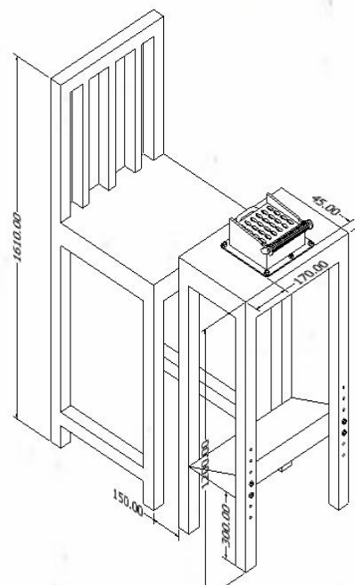
Figure 8 Ergonomically designed work table and seat
