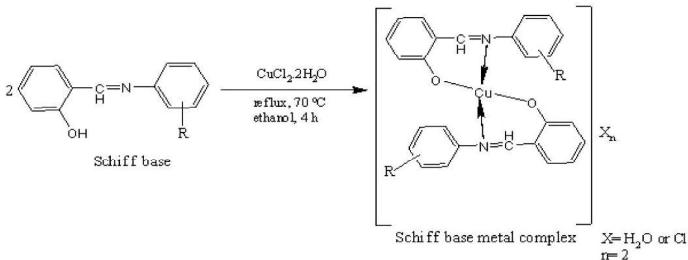
Scheme 2: Synthetic Route to Schiff Base Metal Complexes \text{Cu L}^1 - \text{Cu L}^3
